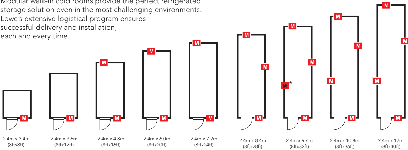
Doors can be added on the long side also. *additional monoblock units for the freezer
